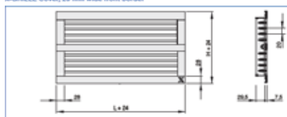
X-GRILLE Cover, 28 mm wide front border
